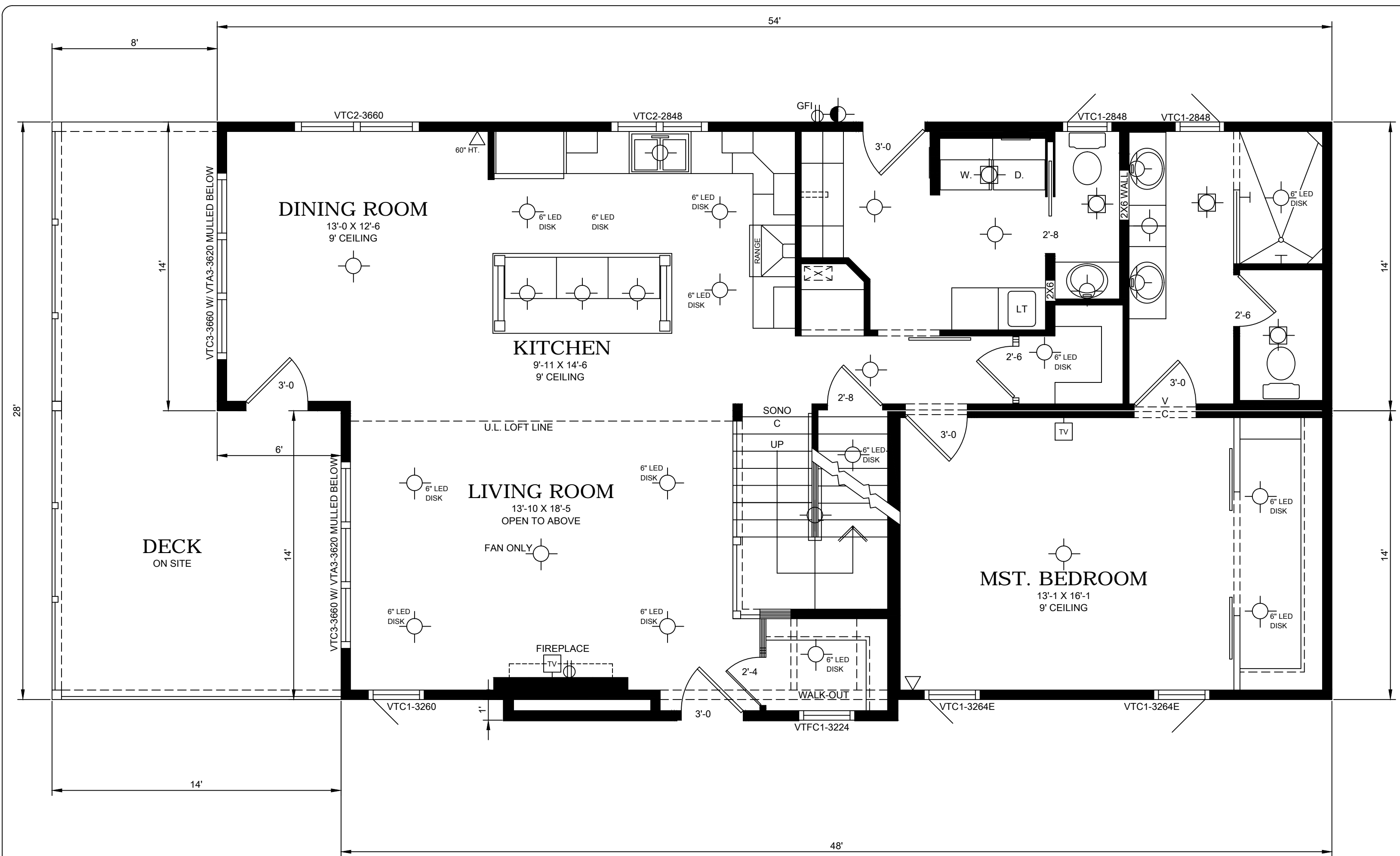
FLOOR PLAN 1/4"=1'-0" (DIMENSIONS FRAMING TO FRAMING)
