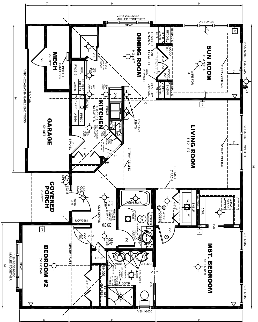
FLOOR PLAN 1/4" = 1'-0" (DIMENSIONS FRAMING TO FRAMING)
